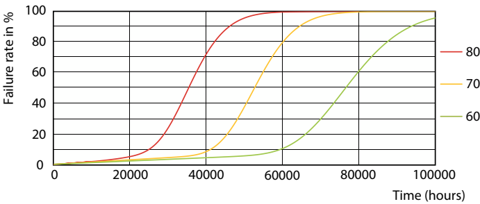
LEDtube-75K-6080-FailureRate-LED
