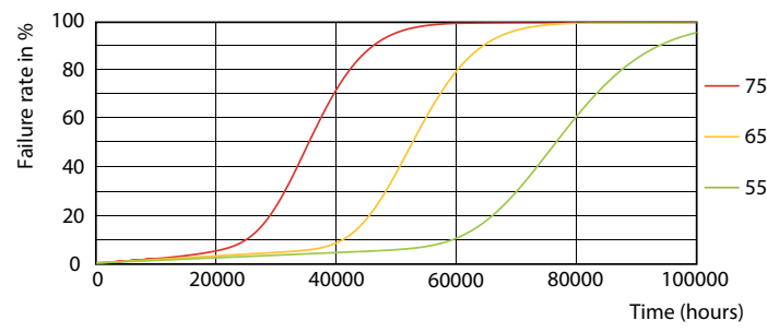
LEDtube-75K-5575-FailureRate-LED
